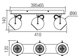
04-544 GU10, 3 x max.35W IP20 230V 50Hz
