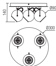
04-545 GU10, 3 x max.35W IP20 230V 50Hz
